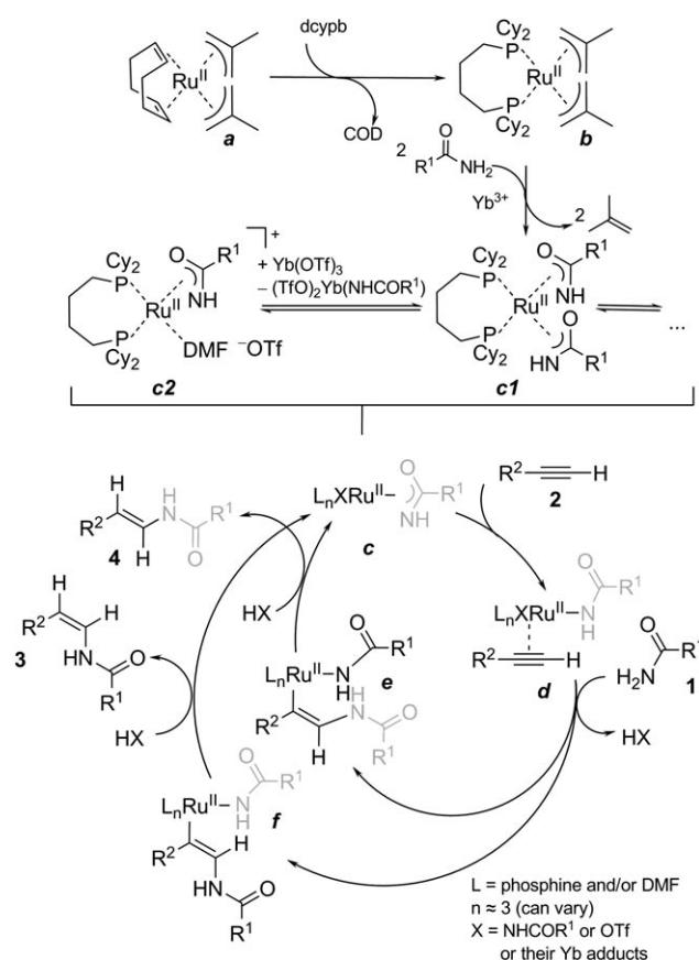
Scheme 2. Proposed reaction mechanism.
