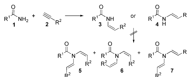
Scheme 1. Stereo- and chemoselectivity in hydroamidations.
